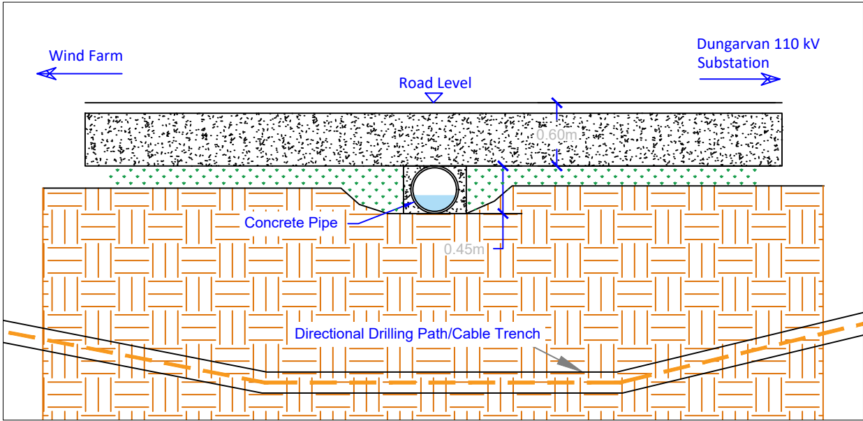
Section B-B
